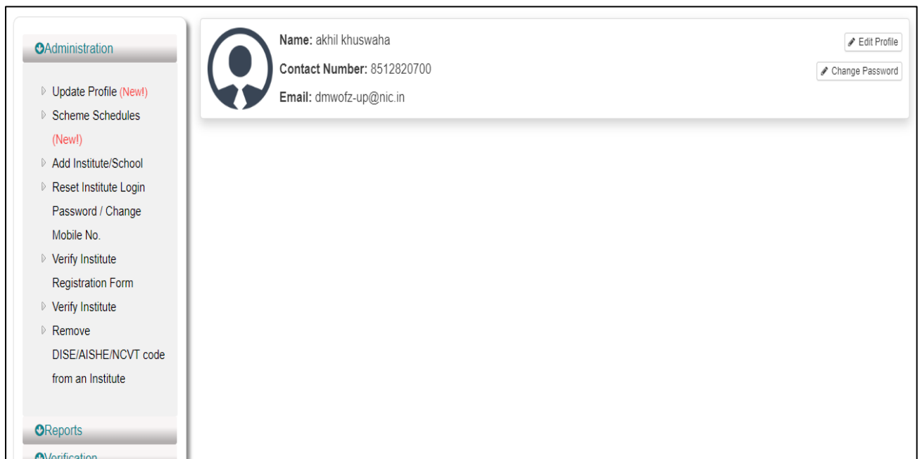
Screen -1
